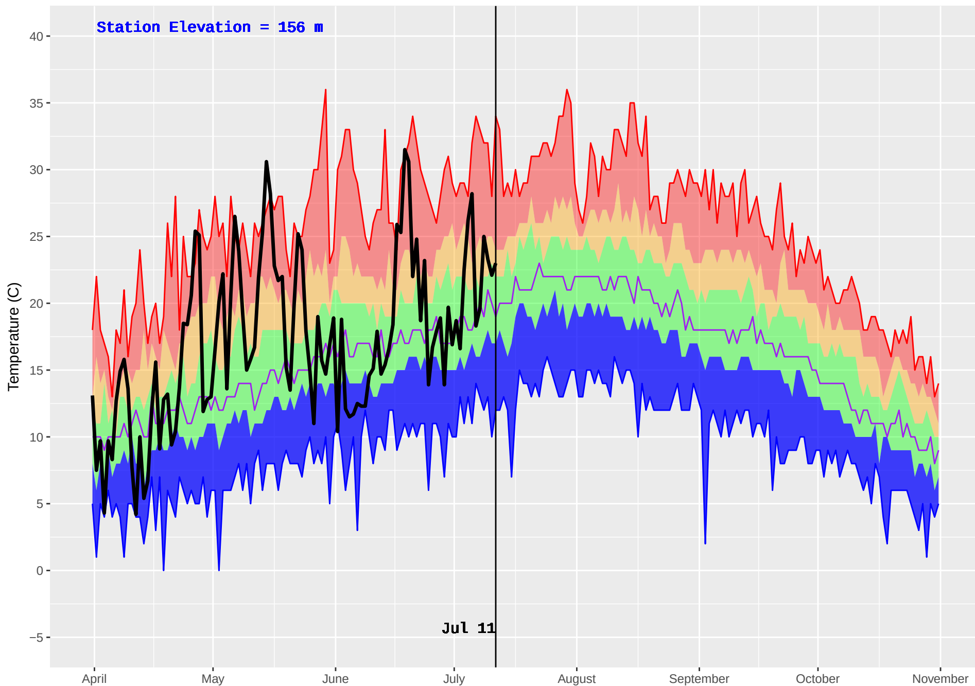
WOSS CAMP (21) : Historical (1970–2016) and Current (2018) Noon Temperature
