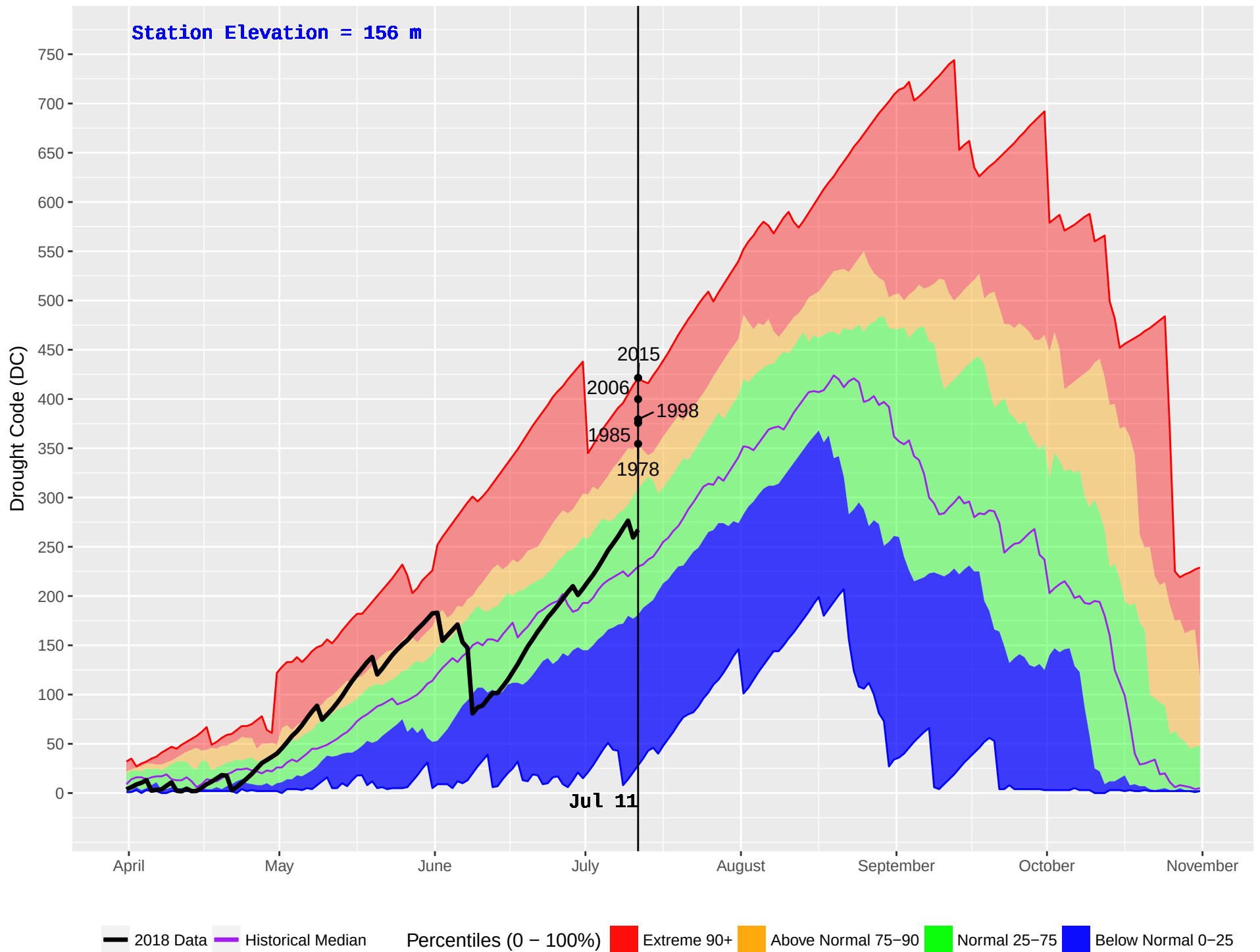
WOSS CAMP (21) : Historical (1970–2016) and Current (2018) Noon Drought Code (DC)
