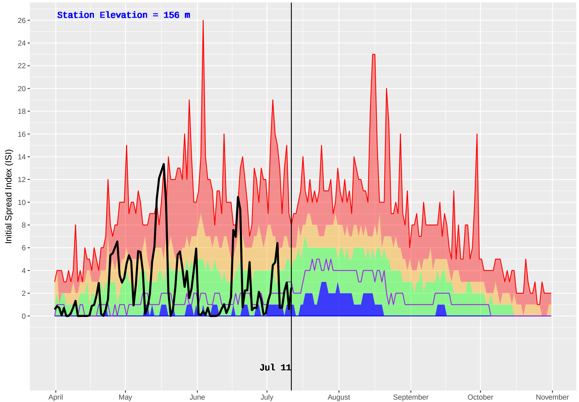
WOSS CAMP (21) : Historical (1970–2016) and Current (2018) Noon Initial Spread Index (ISI)
